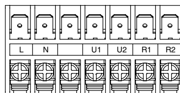
7P terminal board
